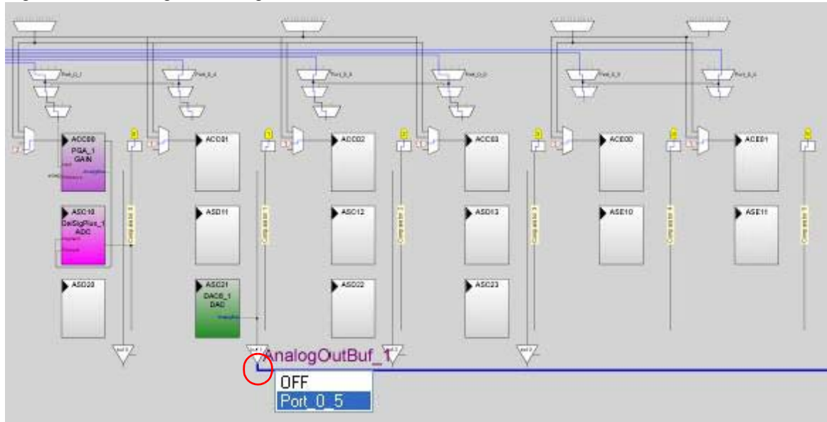
Figure 3-34. Configure AnalogOutBuf_1
