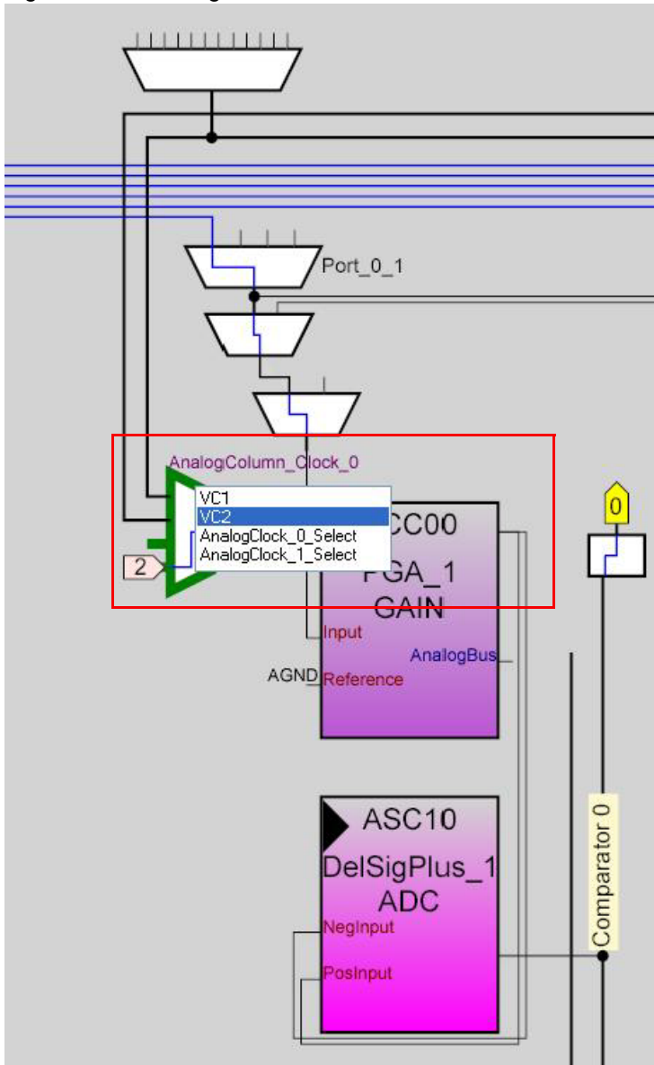
Figure 3-36. AnalogColumn_Clock_0 Connection
